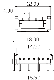
LCDMR-7P4TW
