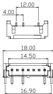
LCDMR-7P3TW
